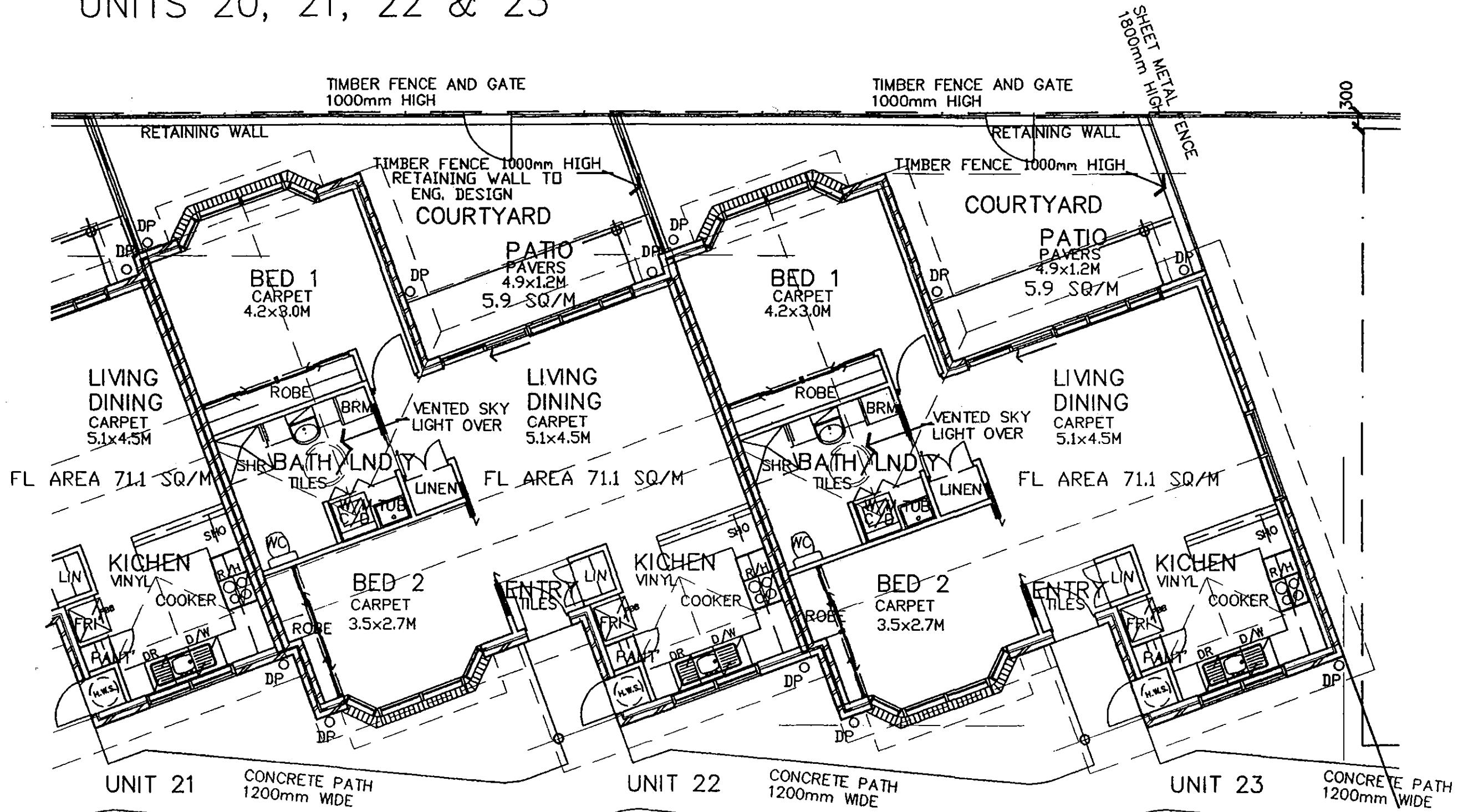
BLOCK G GROUND FLOOR UNITS 20, 21, 22 & 23
